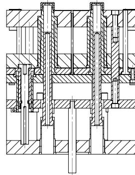
SECTION C-C
