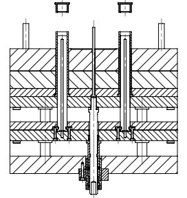
SECTION D-D SECOND EJECTOR STROKE
