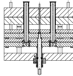
SECTION C-C FIRST EJECTOR STROKE
