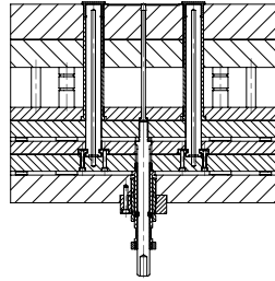
SECTION B-B EJECTOR PLATES BACK - MOLD OPEN
