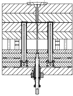
SECTION A-A EJECTOR PLATES BACK - MOLD CLOSED
